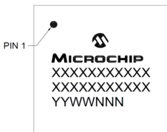
64-Lead TQFP (10x10 mm)
