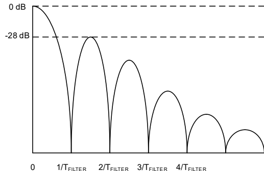
Filter Frequency Response
