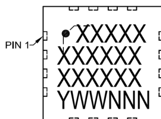
28-Lead VQFN (4x4 mm)
