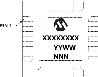
20-Lead VQFN
