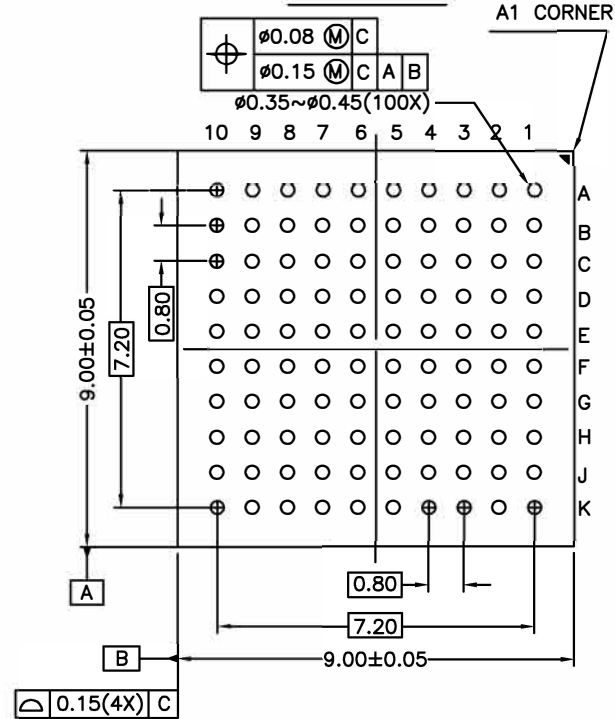
BOTTOM VIEW
