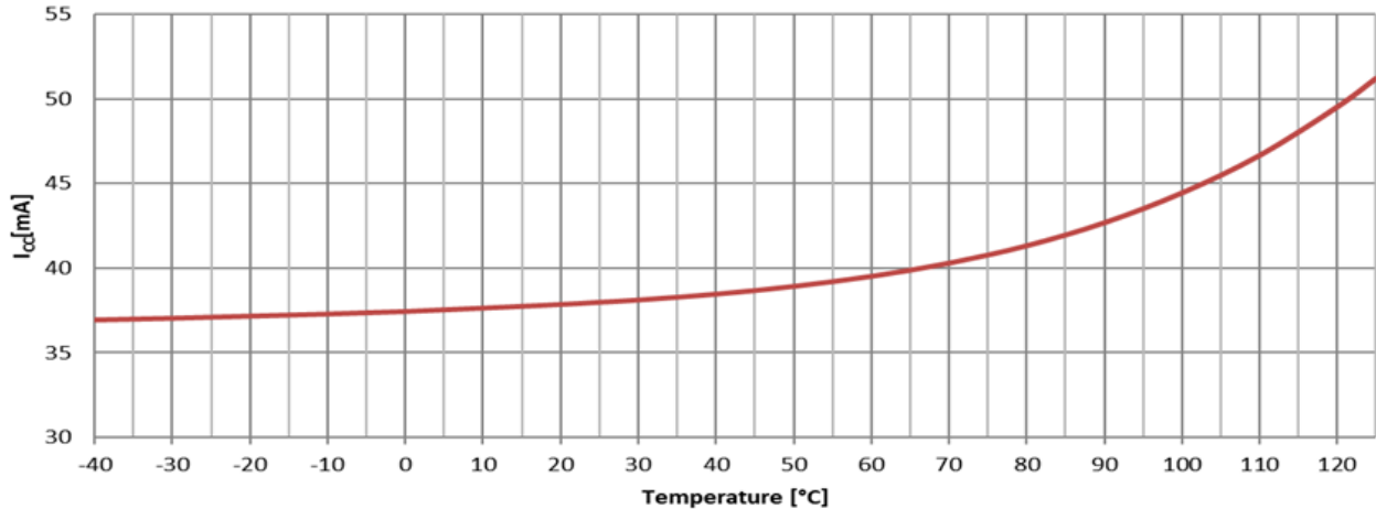
Consumption Coremark
