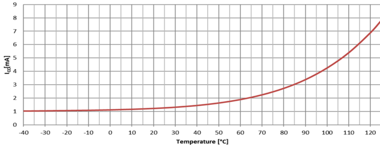
Consumption Standby - VDDCOREx = 0.8 V
