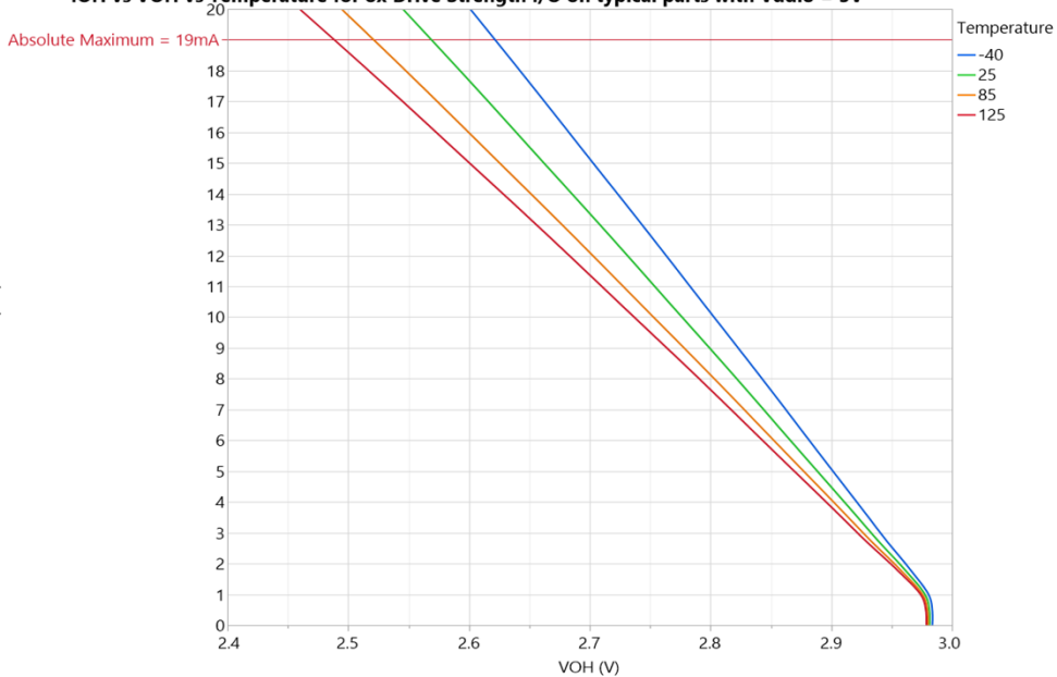
IOH vs VOH vs Temperature for 8x Drive Strength I/O on typical parts with Vddio = 3V
