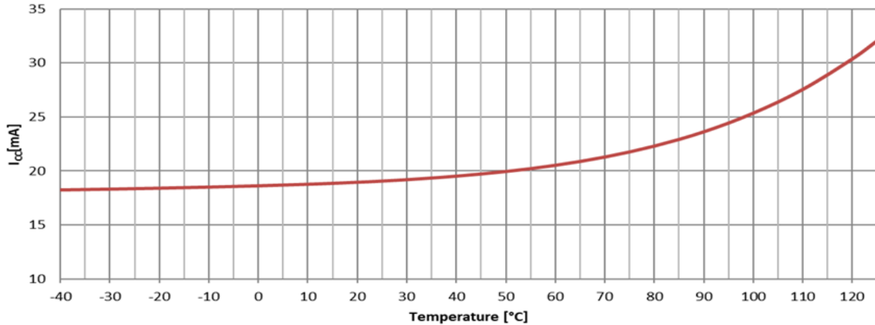
Consumption Idle
