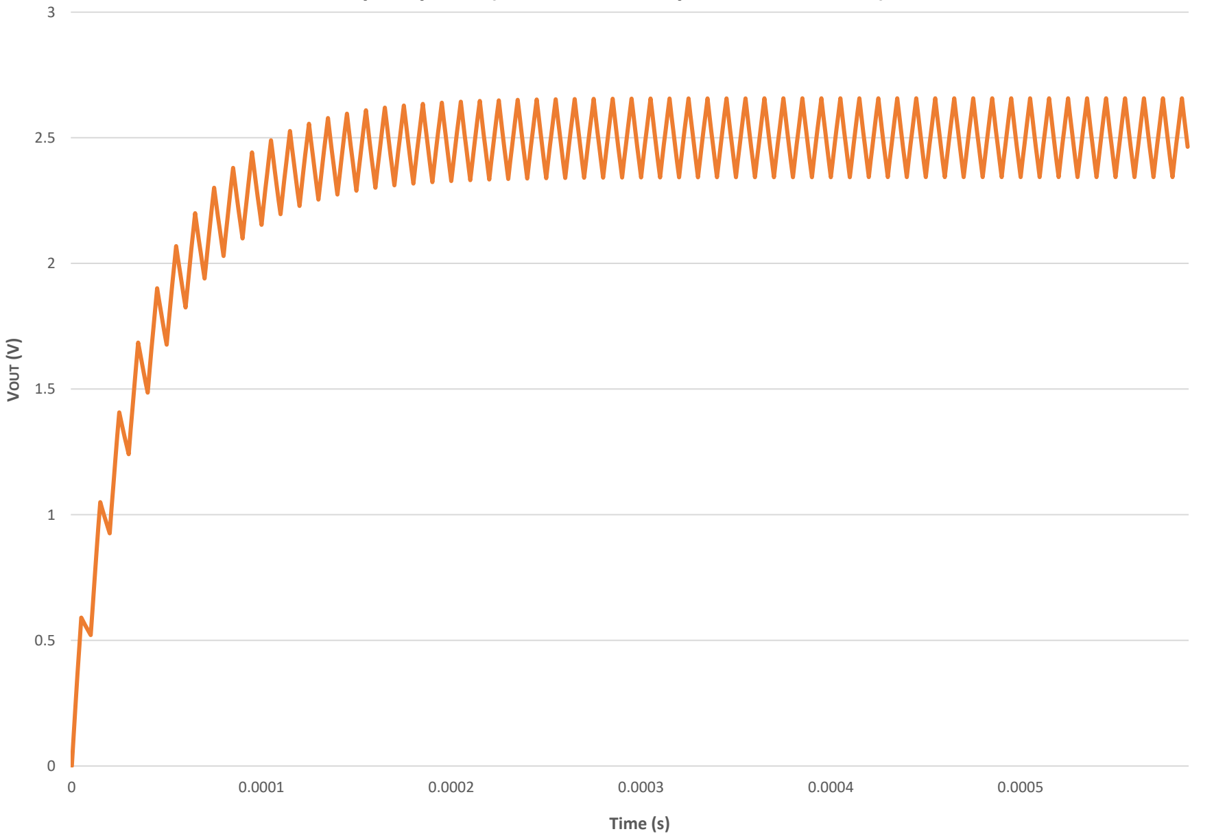
Step Response ( R = 40 \text{ M}\Omega , C = 1 \text{ pF} , F_{\text{PWM}} = 100 \text{ kHz} )
