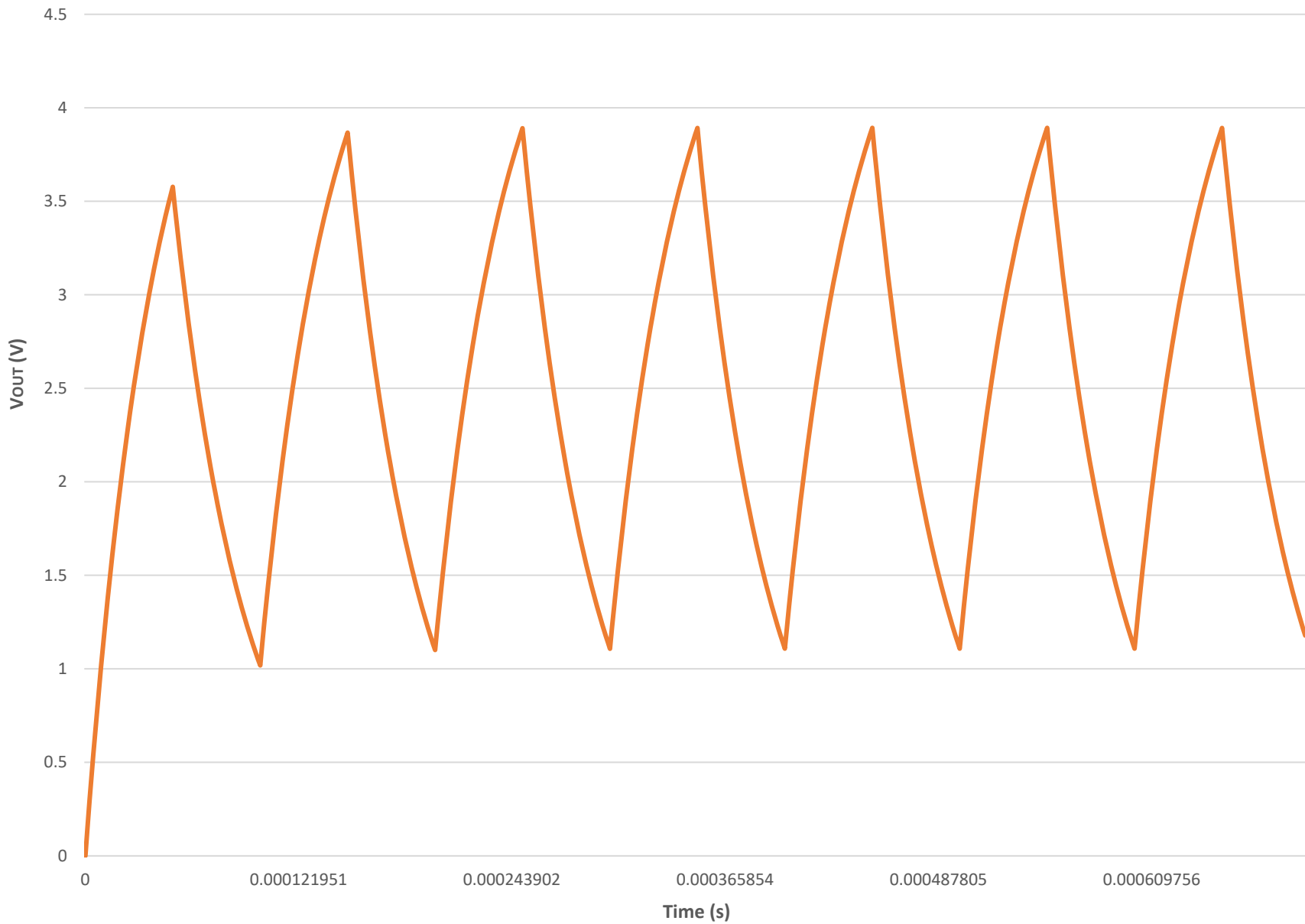
Step Response ( R = 1.8\text{ k}\Omega , C = 0.022\text{ }\mu\text{F} , F_{\text{PWM}} = 10\text{ kHz} )
