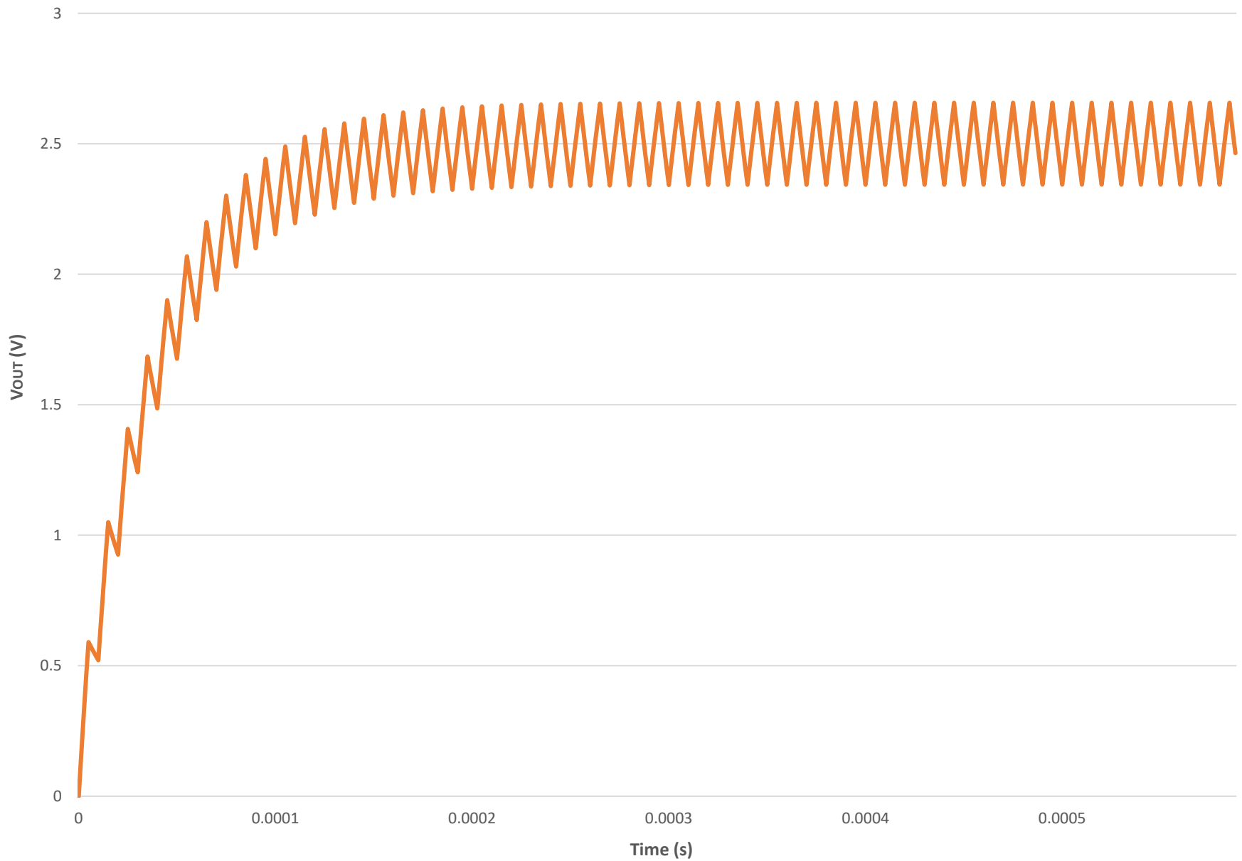
Step Response ( R = 4 \text{ k}\Omega , C = 0.01 \text{ }\mu\text{F} , F_{\text{PWM}} = 100 \text{ kHz} )
