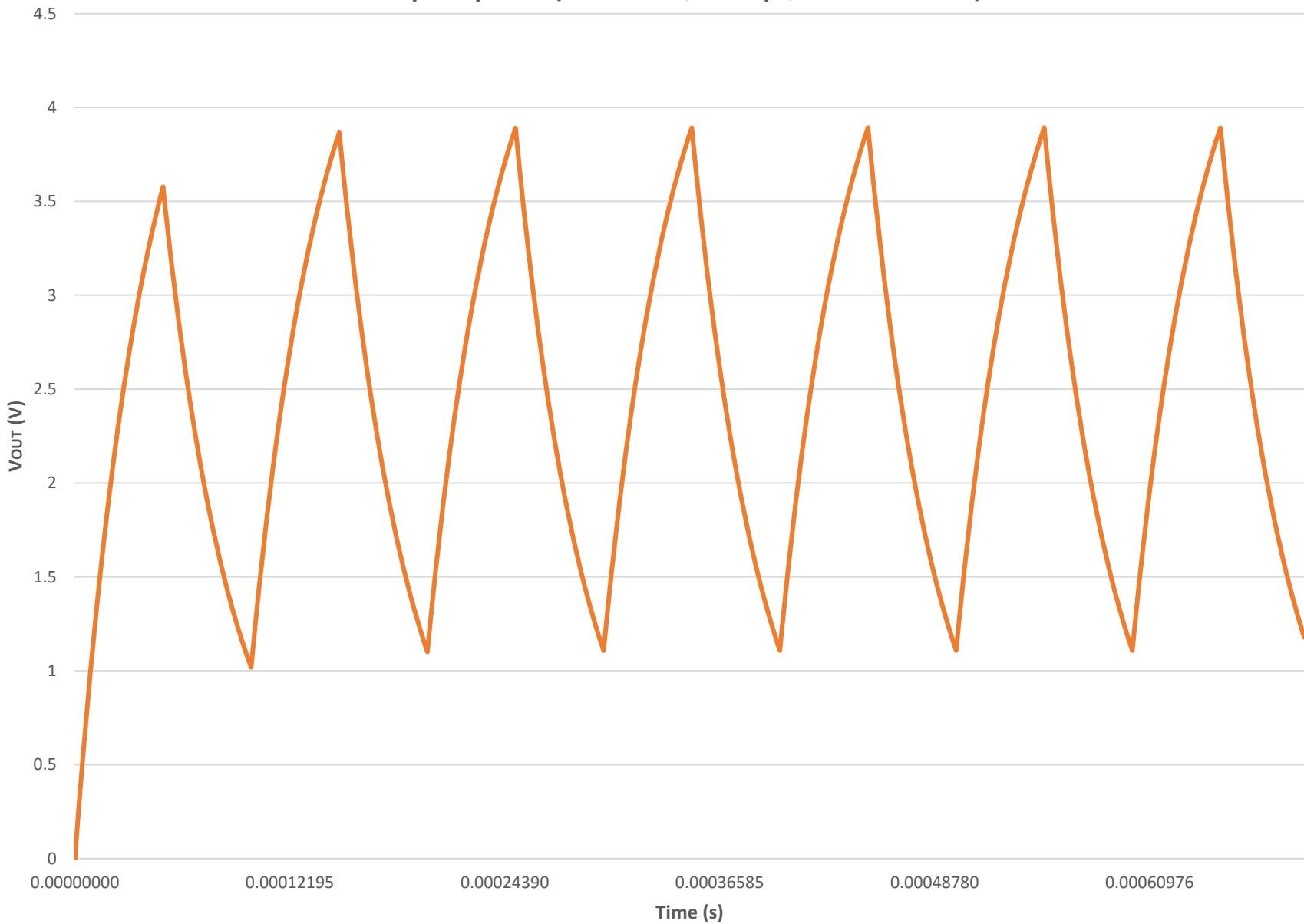
Step Response ( R = 40 \text{ M}\Omega , C = 1 \text{ pF} , F_{\text{PWM}} = 10 \text{ kHz} )
