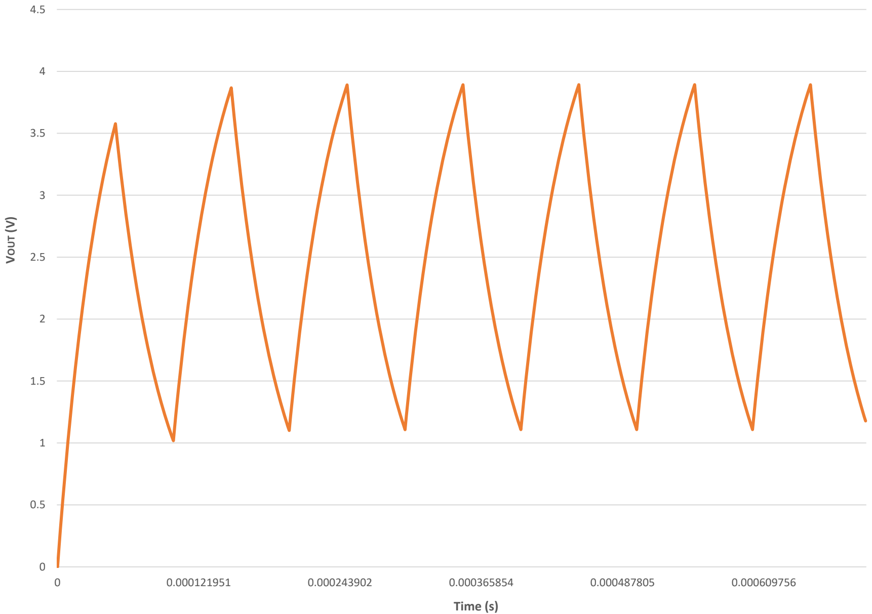
Step Response ( R = 4\text{ k}\Omega , C = 0.01\text{ }\mu\text{F} , F_{\text{PWM}} = 10\text{ kHz} )
