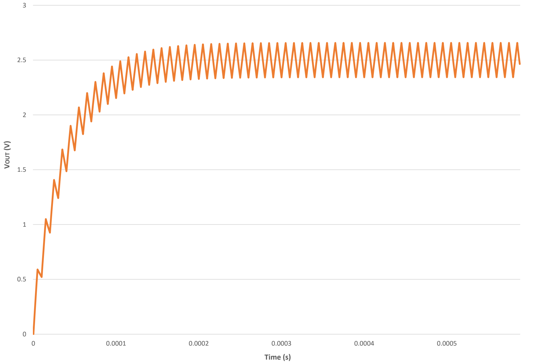
Step Response ( R = 1.8 \text{ k}\Omega , C = 0.022 \text{ }\mu\text{F} , F_{\text{PWM}} = 100 \text{ kHz} )
