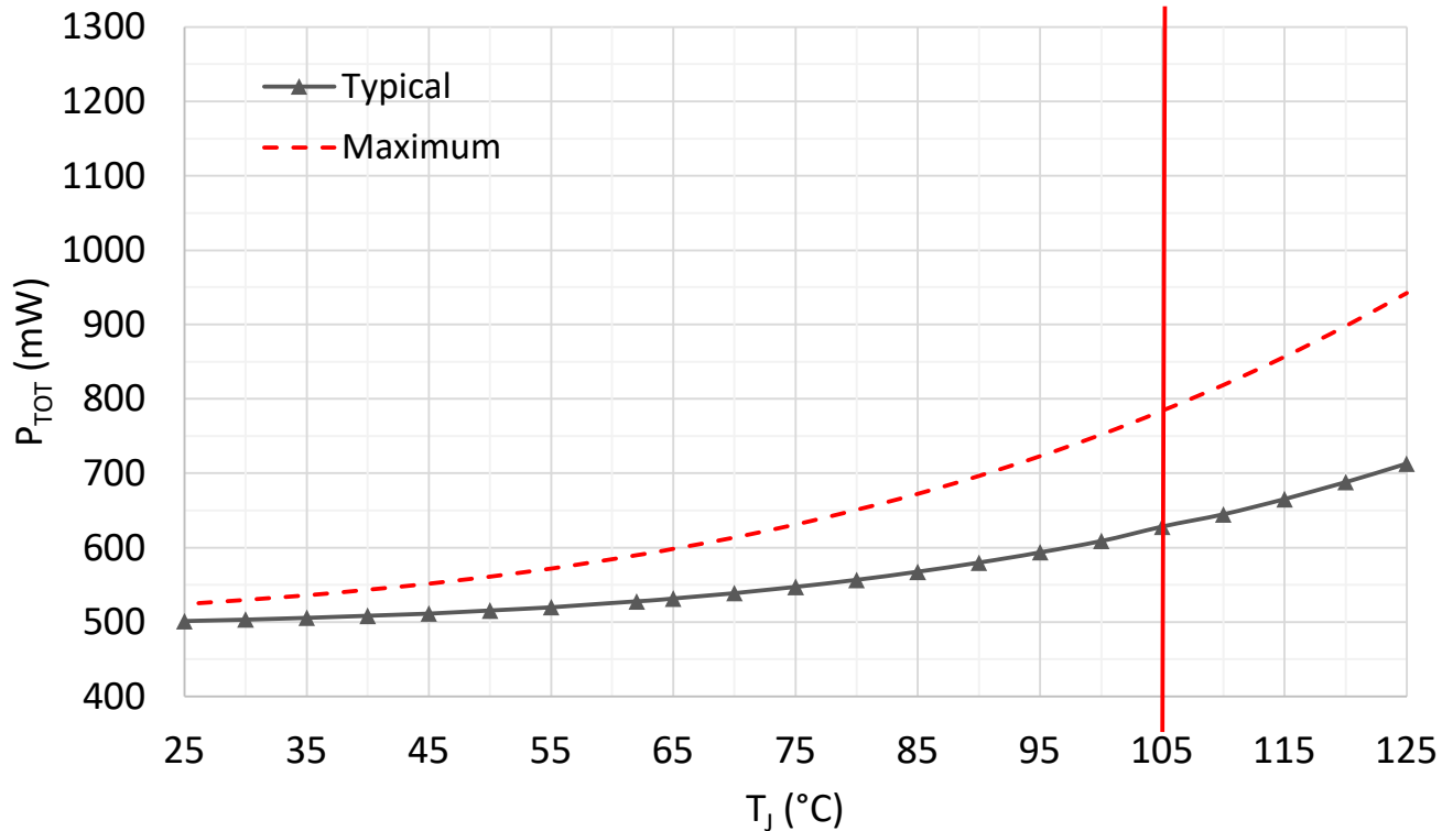
Use Case 1: P_{TOT} vs T_J
