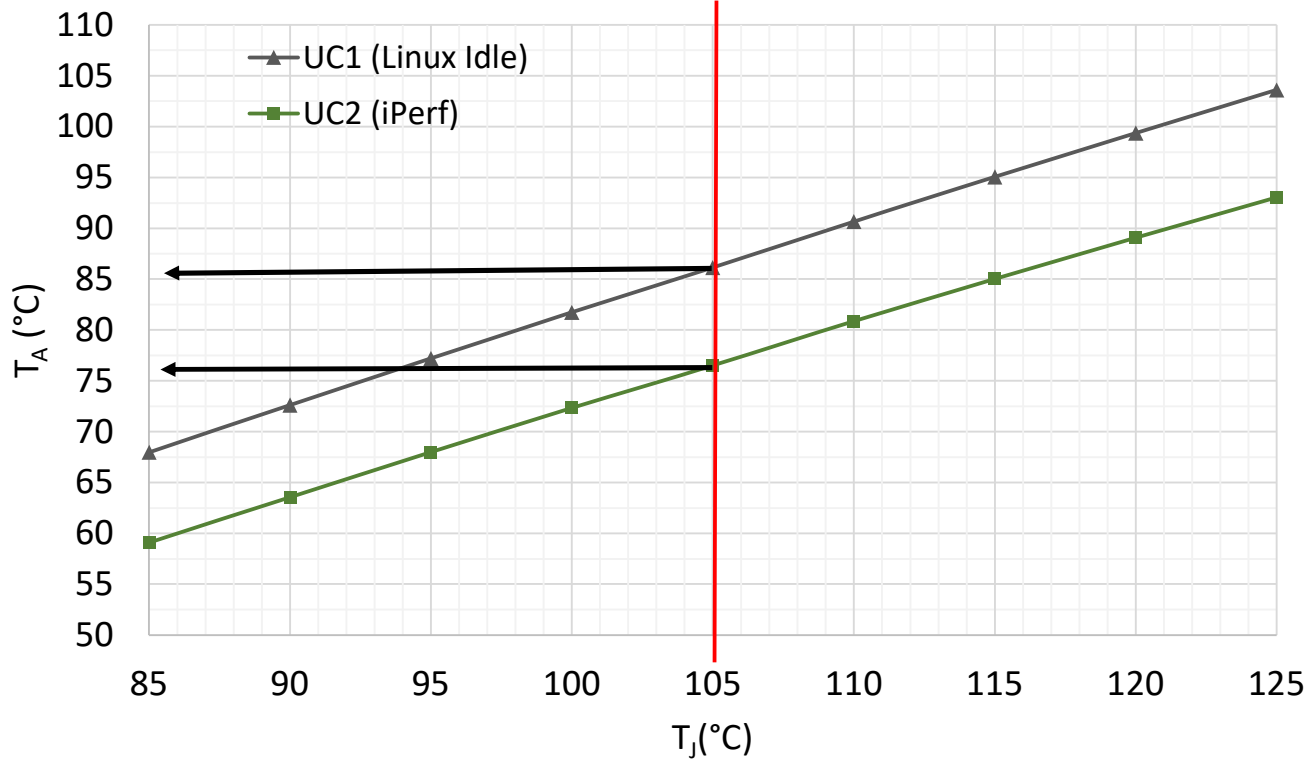
Use Cases 1 & 2: T_A vs T_J
