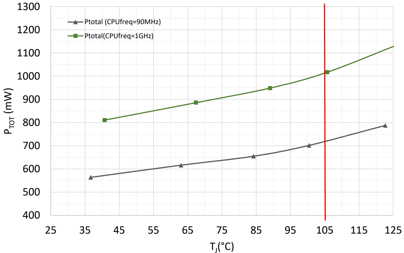
Max P_{TOT} vs T_J
