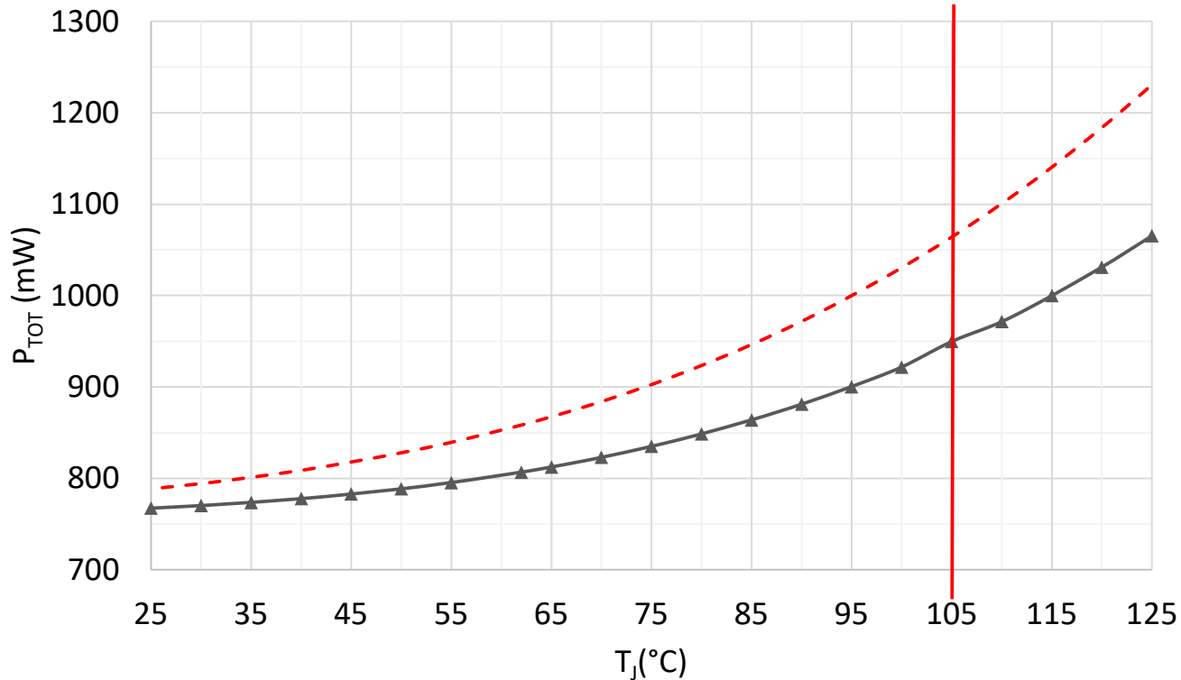
Use Case 2: P_{TOT} vs T_J
