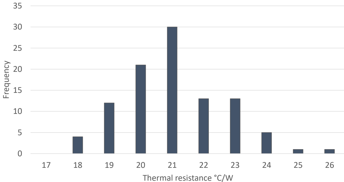
Thermal resistance distribution of SAMA7G5 SiP, average=20.5°C/W
