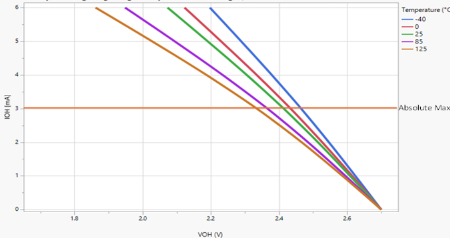
Output voltage High: High sink pins in Low Strength, DRVSTR=0 with Vddio 2.7V
