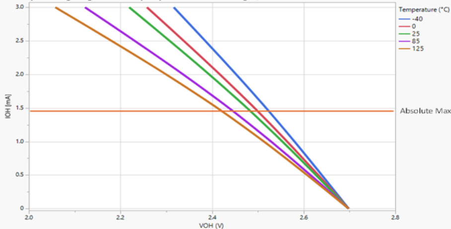
Output voltage High: Standard pins pins in Low Drv Strength, DRVSTR=0 with Vddio 2.7V
