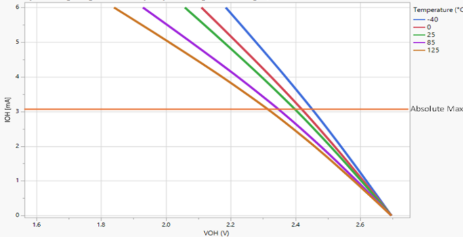
Output voltage High: Standard pins pins in High Drv Strength, DRVSTR= 1 with Vddio 2.7V
