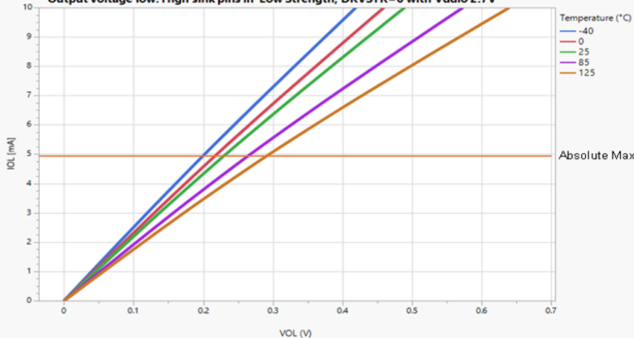
Output voltage low: High sink pins in Low Strength, DRVSTR=0 with Vddio 2.7V
