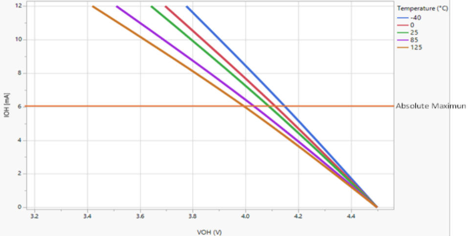
Output voltage High: High sink pins in Low Strength, DRVSTR=0 with Vddio 4.5V
