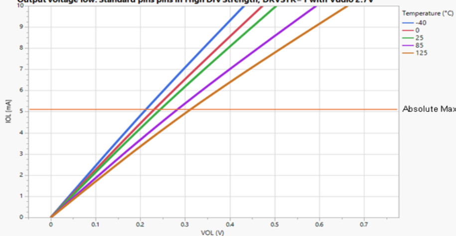
Output voltage low: Standard pins pins in High Drv Strength, DRVSTR= 1 with Vddio 2.7V
