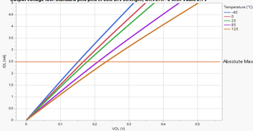
Output voltage low: Standard pins pins in Low Drv Strength, DRVSTR=0 with Vddio 2.7V
