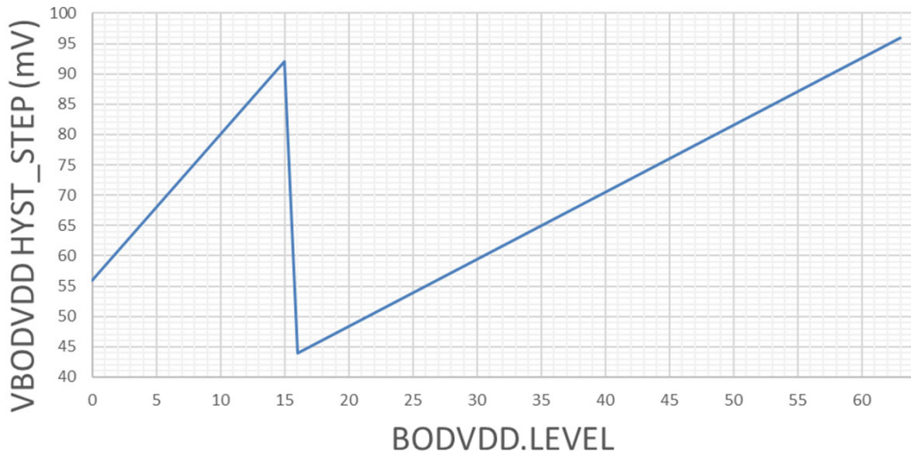
VBODVDD HYST_STEP (mV) versus BODVDD.LEVEL
