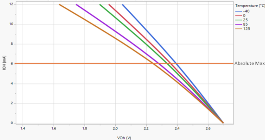
Output voltage High: High sink pins in High Strength, DRVSTR=1 with Vddio 2.7V
