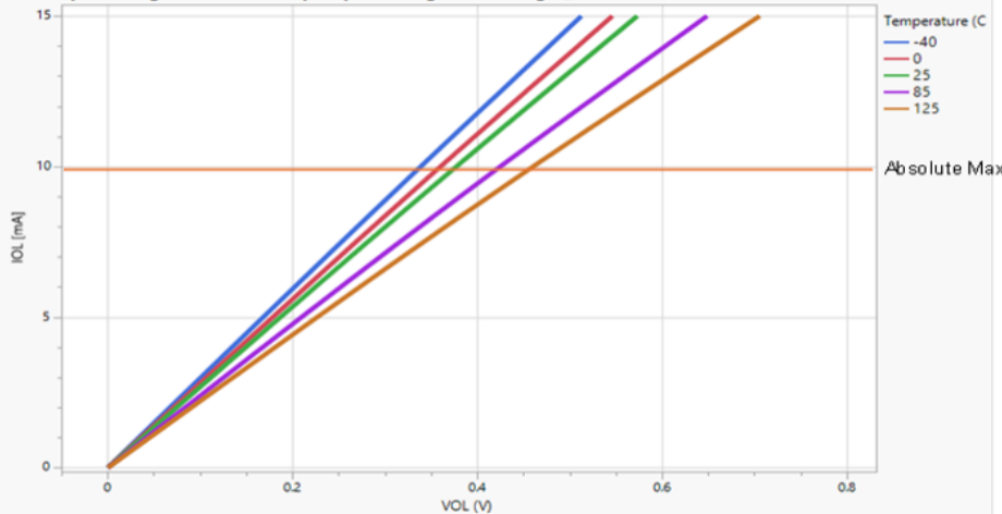
Output voltage low: Standard pins in High Drv Strength, DRVSTR=1 with Vddio 4.5V
