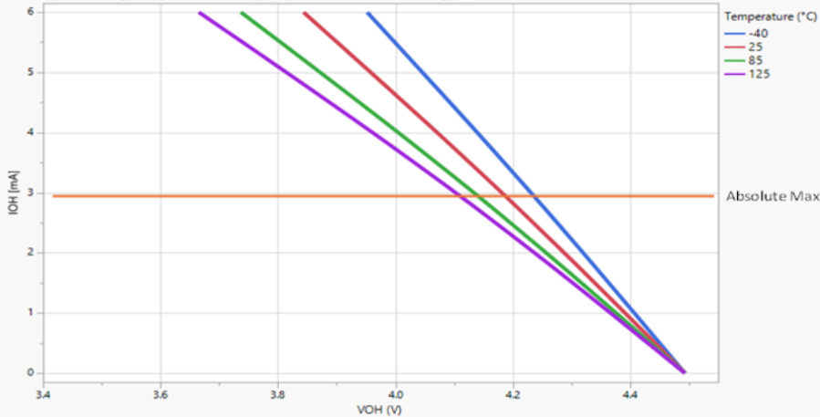
Output voltage High: Standard pins pins in Low Drv Strength, DRVSTR=0 with Vddio 4.5V
