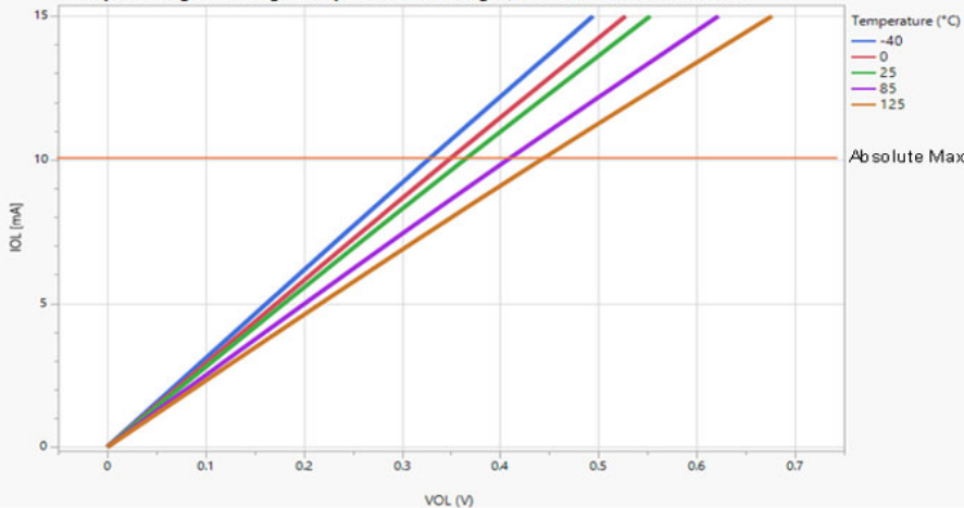
Output voltage low: High sink pins in Low Strength, DRVSTR=0 with Vddio 4.5V
