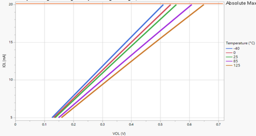
Output voltage low: High sink pins in High Strength, DRVSTR= 1 with Vddio 4.5V
