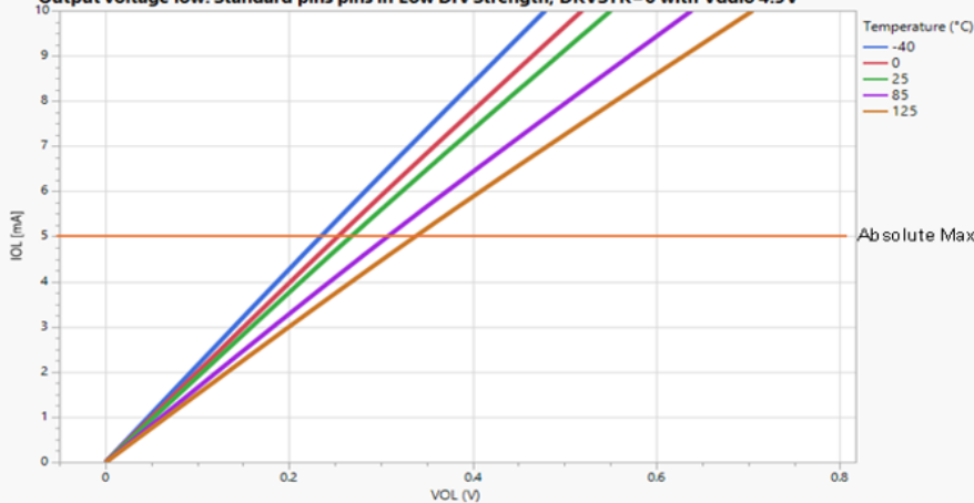
Output voltage low: Standard pins pins in Low Drv Strength, DRVSTR=0 with Vddio 4.5V
