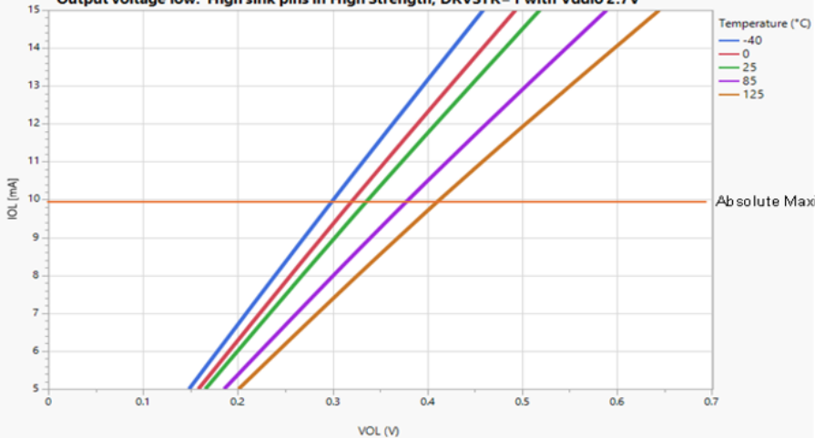
Output voltage low: High sink pins in High Strength, DRVSTR= 1 with Vddio 2.7V
