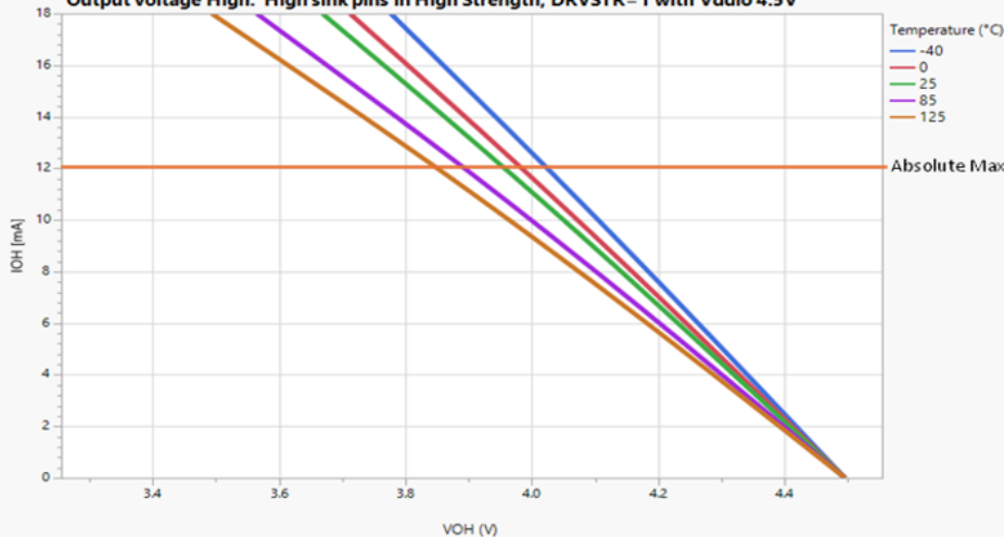
Output voltage High: High sink pins in High Strength, DRVSTR=1 with Vddio 4.5V
