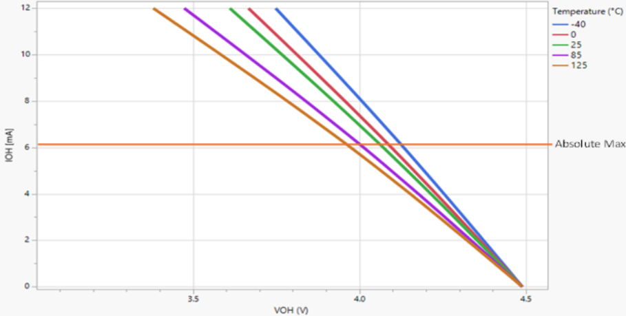
Output voltage High: Standard pins pins in High Drv Strength, DRVSTR= 1 with Vddio 4.5V
