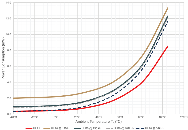
Typical Power Consumption in ULP0 and ULP1 vs Ambient Temperature ( T_A )
