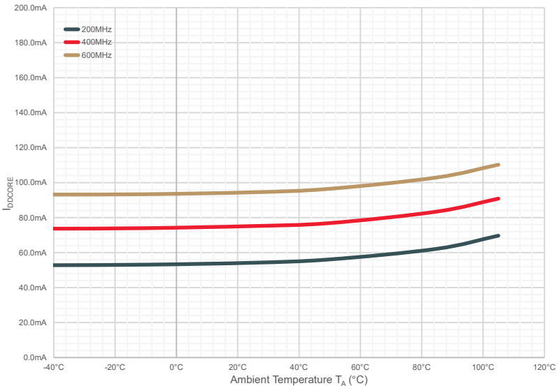
Processor Current Consumption in Active Mode
