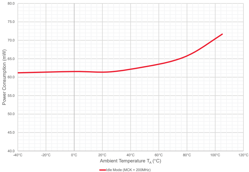
Typical Power Consumption in Idle Mode vs Ambient Temperature ( T_A )
