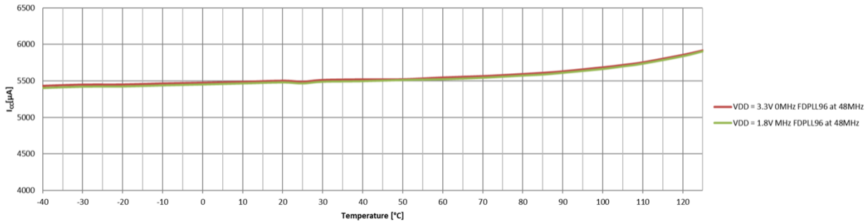
Coremark Typ Power Consumption PL2 48MHz
