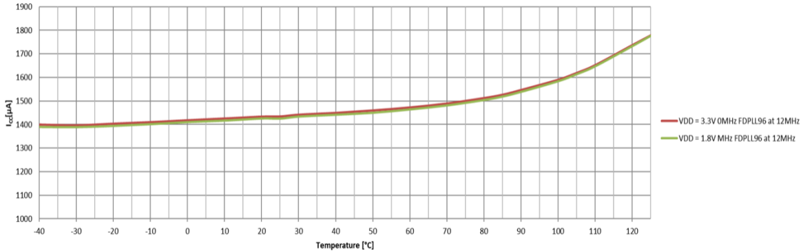
Coremark Typ Power Consumption PLO 12MHz
