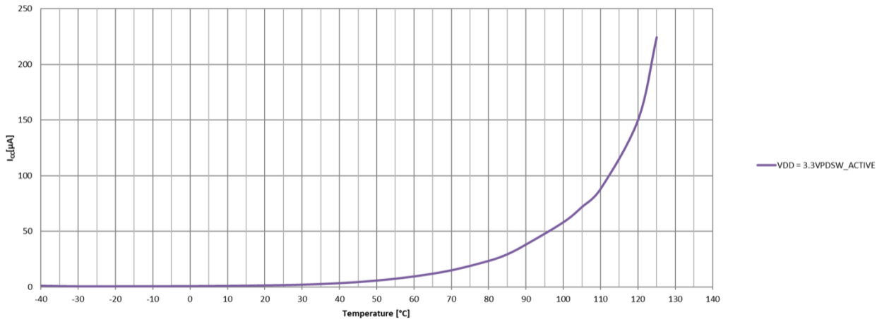
Typical Power Consumption over Temperature in Standby Mode (PDSW Domain Active, 64kB SRAM retained, VREG.LPEFF=1)
