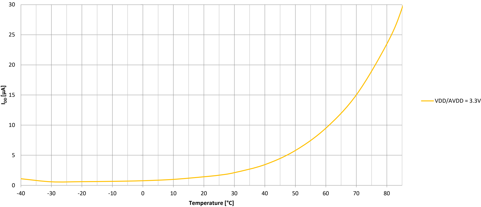
Typical Power Consumption over Temperature in Standby Mode (PDSW Domain Active, 64kB SRAM retained, VREG.LPEFF=1)
