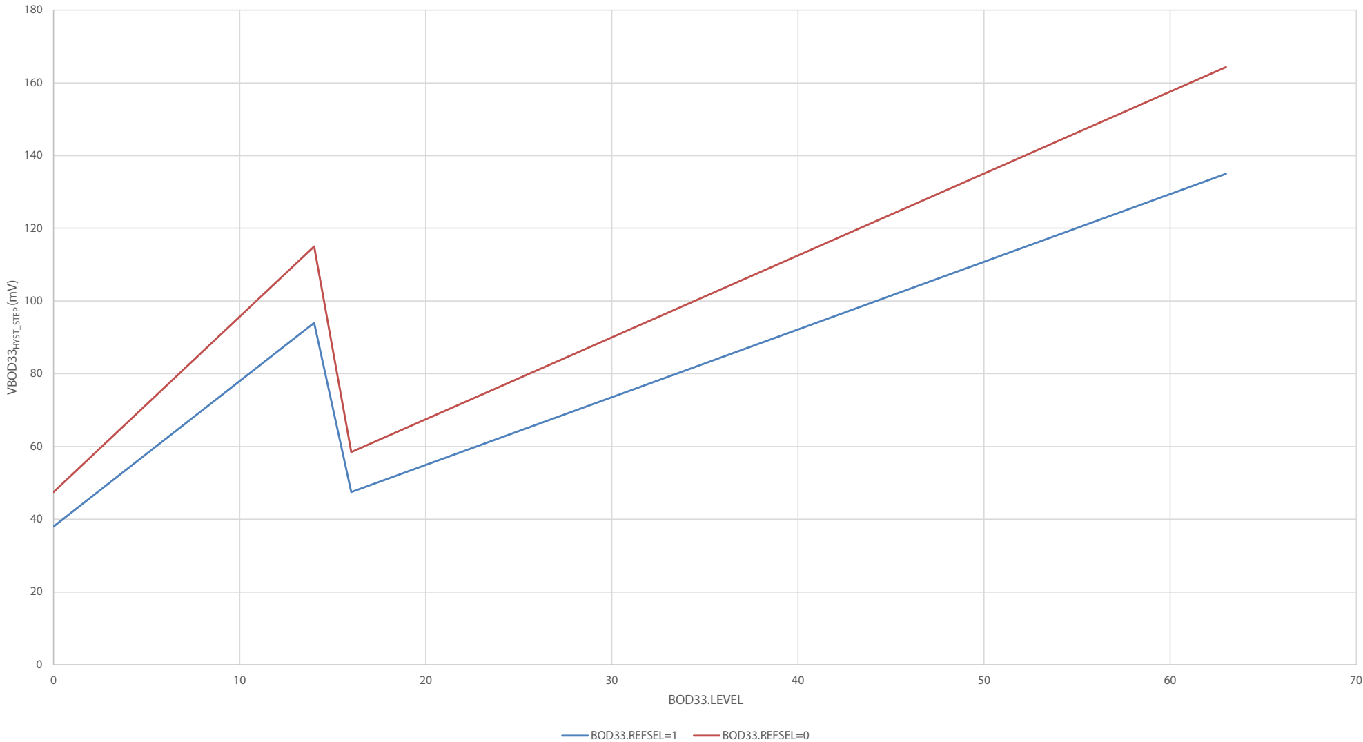
VBOD33 Hysteresis Step (mV) vs. BOD33.LEVEL
