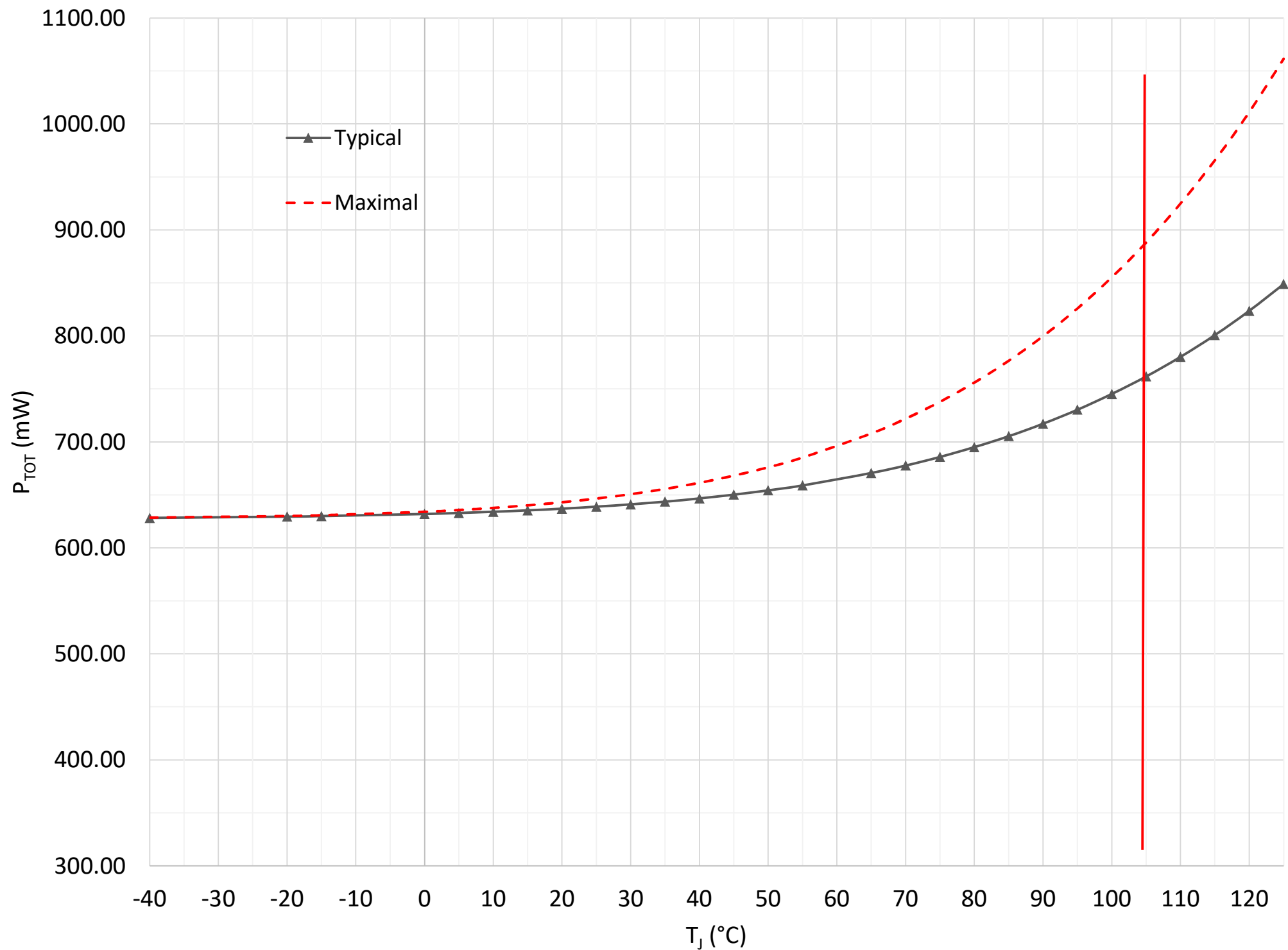
Use case 2 : P_{TOT} vs T_J
