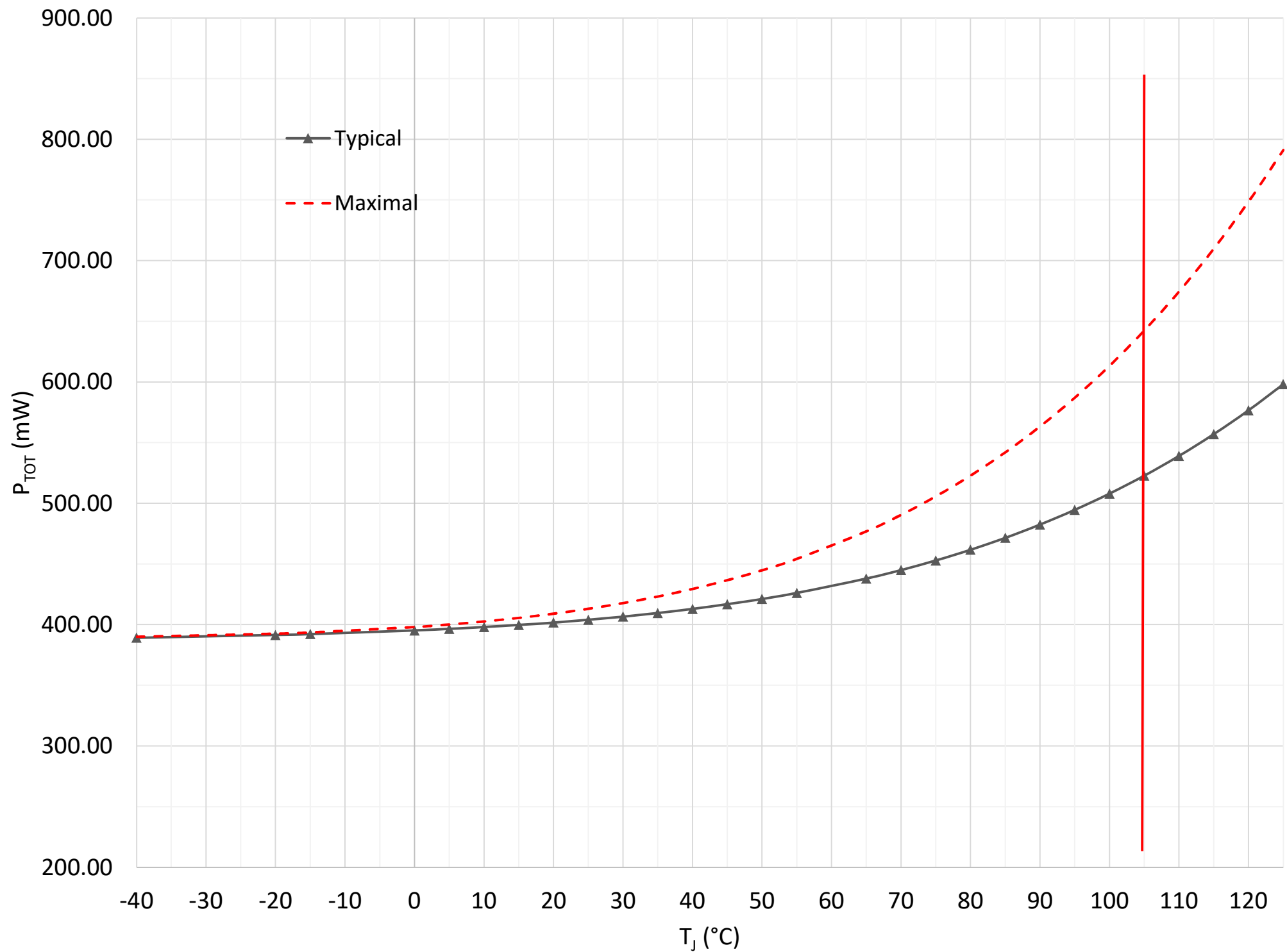
Use case 1 : P_{TOT} vs T_J
