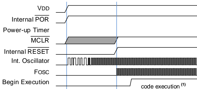
Internal Oscillator, PWRTS = 00
