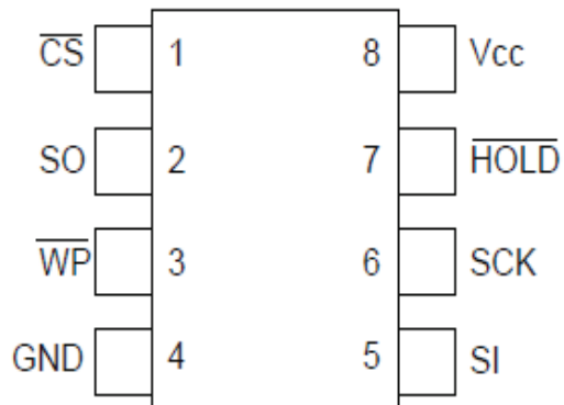
8-Lead SOIC/TSSOP (Top View)
