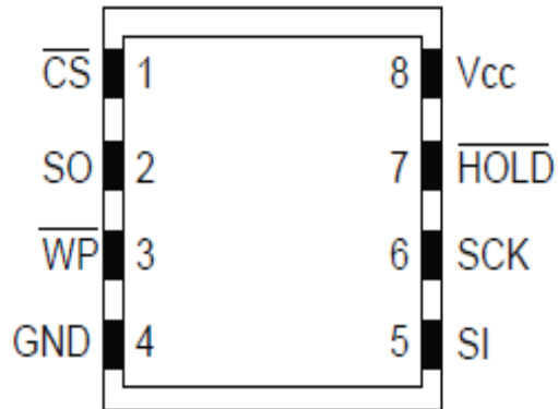
8-Pad UDFN (Top View)
