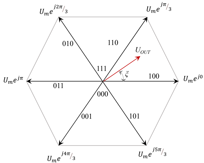
a. Space Vectors for inverter states
